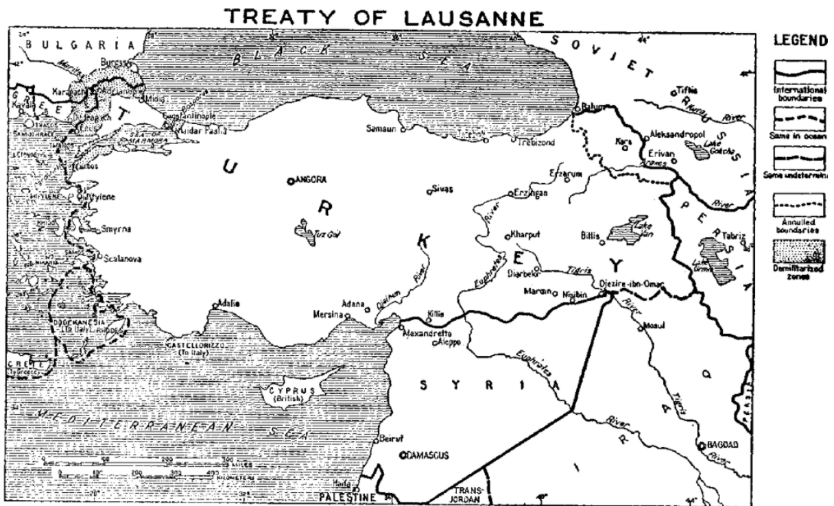
FIGURE 14 TURKEY IN 1923
